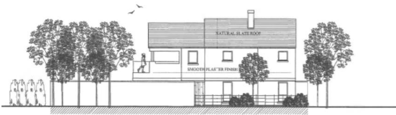
REAR ELEVATION
